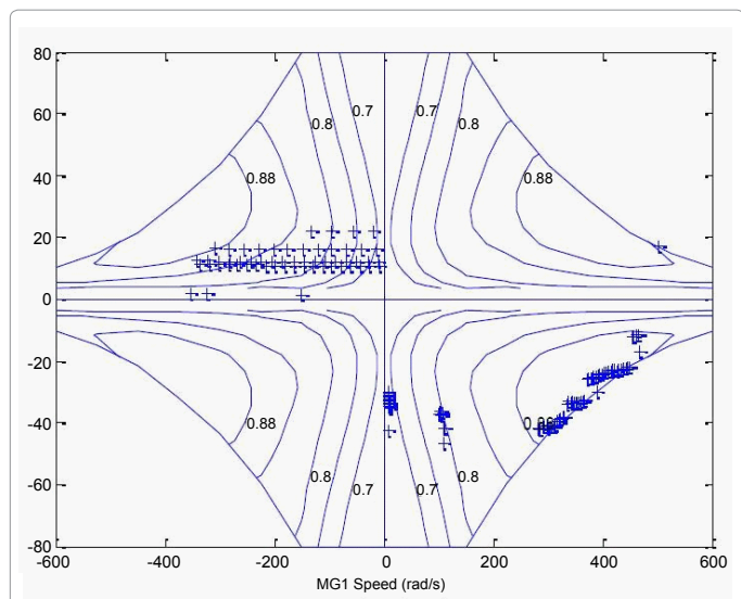
Figure 10: Operation of MG1, twin epicyclic system.
