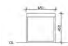
side elevation of seat
