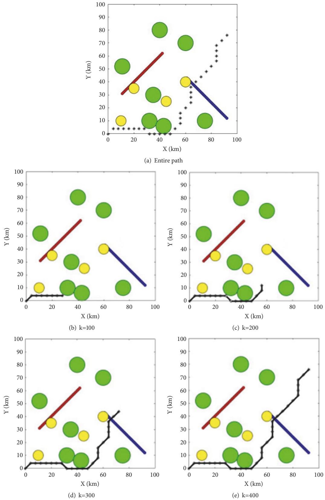
FIGURE 12: UAV path planning in another environment based on our proposed algorithm. And there are both static and mobile threats where (a) is an entire path and (b) to (e) are paths with iterations = 100, 200, 300, 400.
