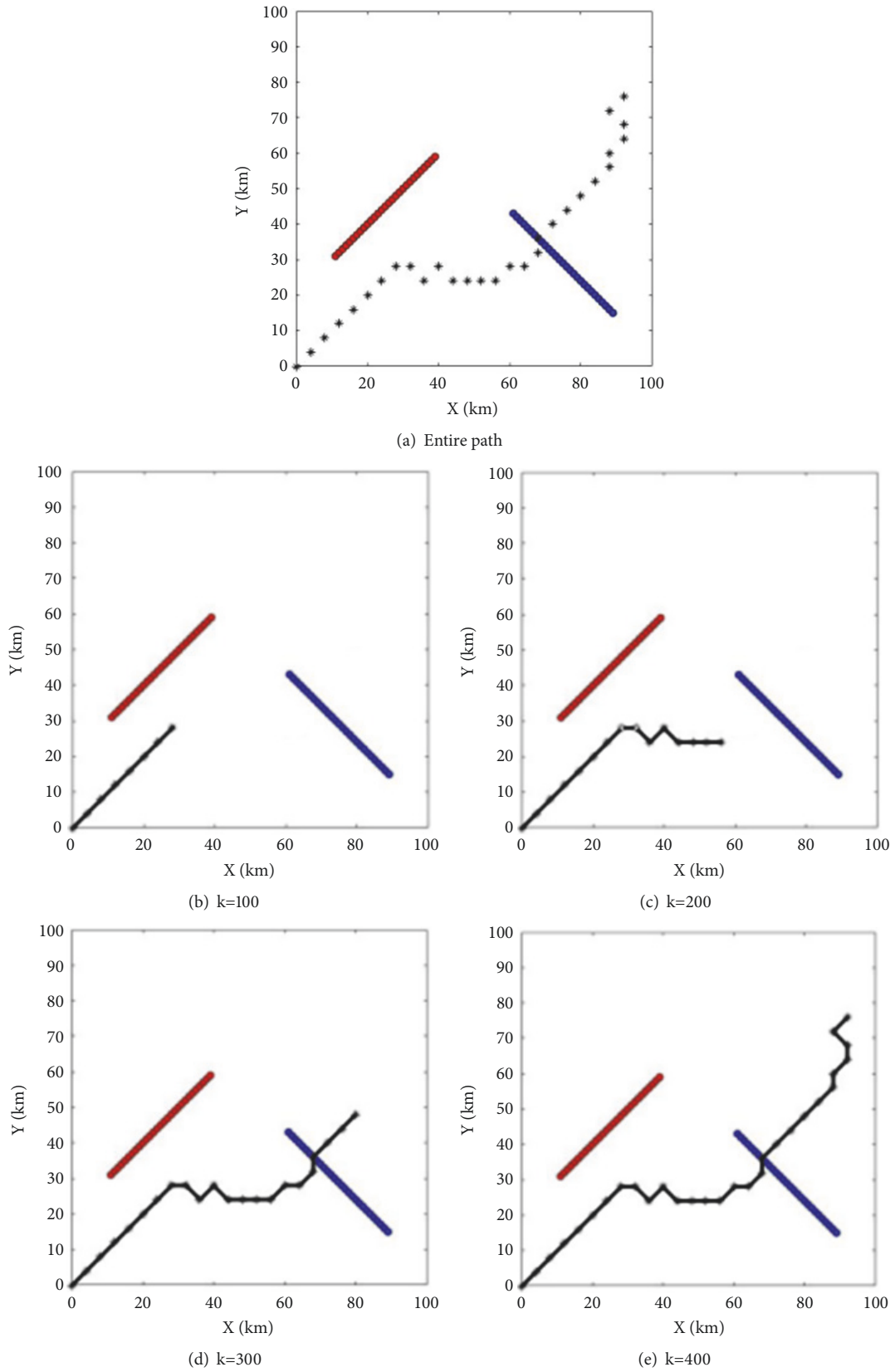
FIGURE 15: UAV path planning in another environment based on ACO algorithm. And there are only mobile threats where (a) is an entire path and (b) to (e) are paths with iterations = 100, 200, 300, 400.
