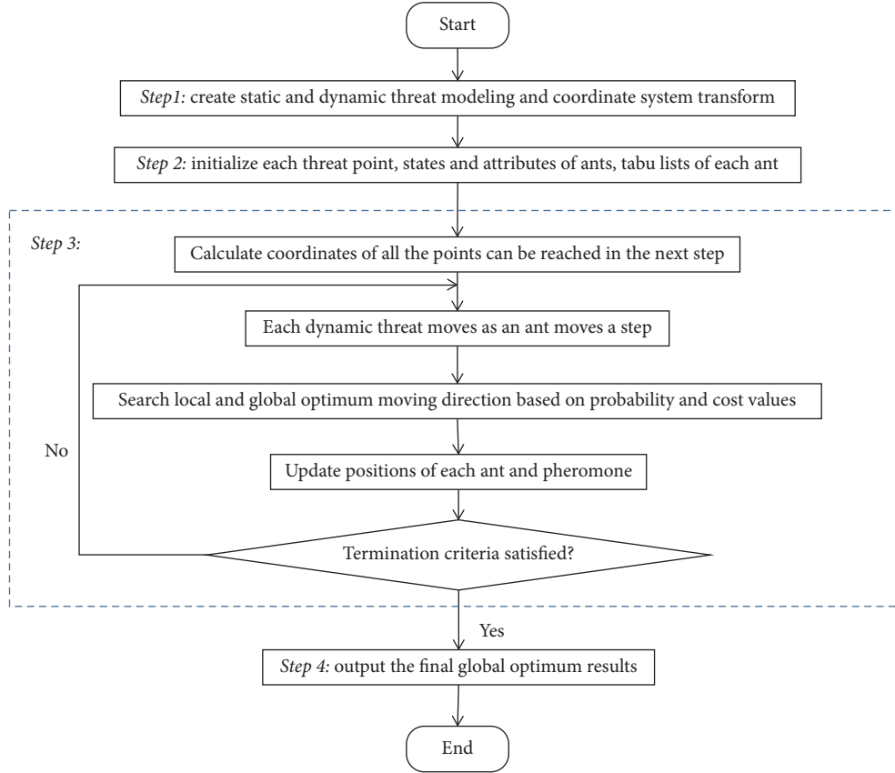
FIGURE 5: Flowchart of the proposed algorithm.
