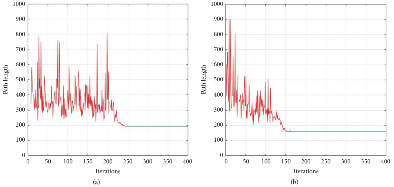
FIGURE 6: The optimal path length with the increase of iterations in one environment. There are both static and mobile threats in (a) and only mobile threats in (b).
