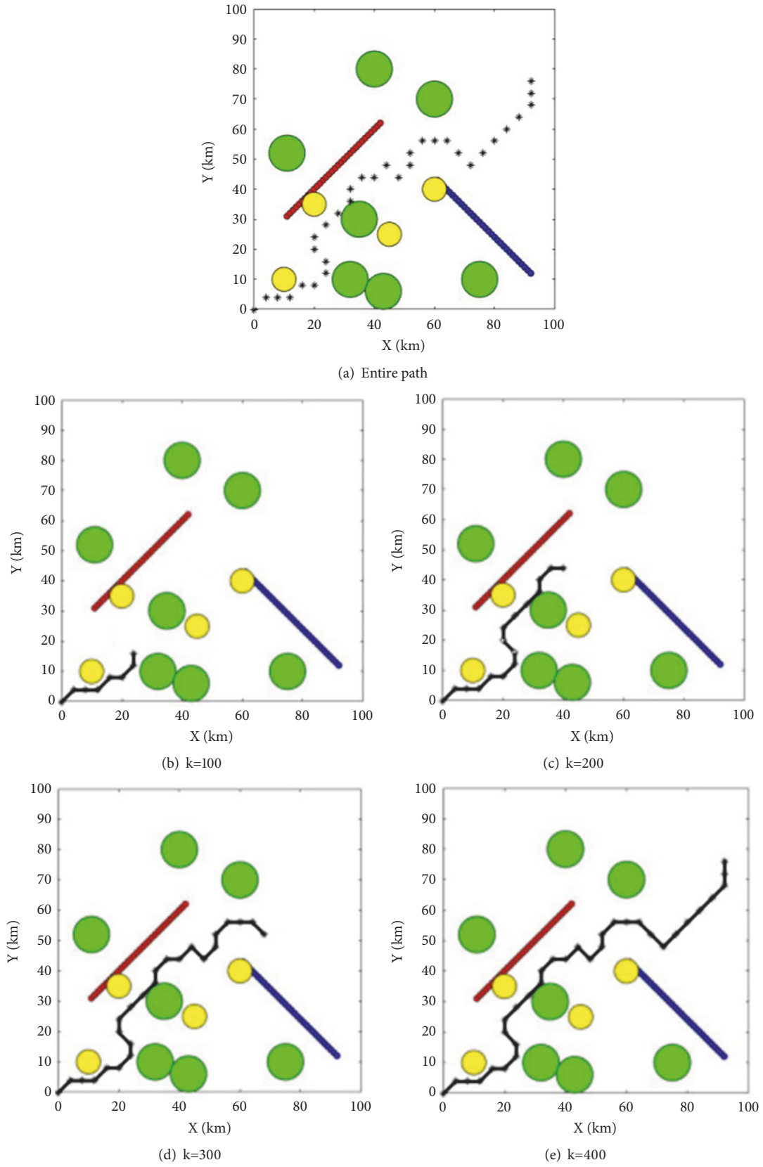
FIGURE 13: UAV path planning in another environment based on ACO algorithm. And there are both static and mobile threats where (a) is an entire path and (b) to (e) are paths with iterations = 100, 200, 300, 400.
