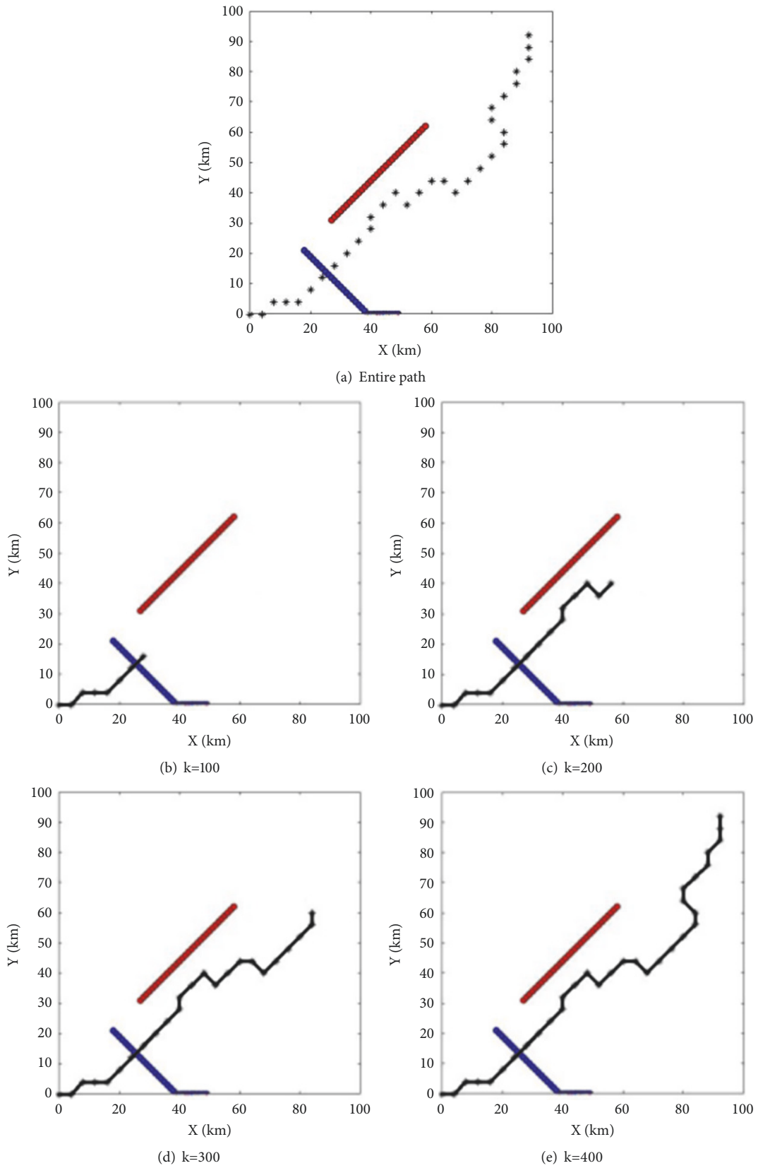
FIGURE 10: UAV path planning in one environment based on our proposed algorithm. And there are only mobile threats where (a) is an entire path and (b) to (e) are paths with iterations = 100, 200, 300, 400.
