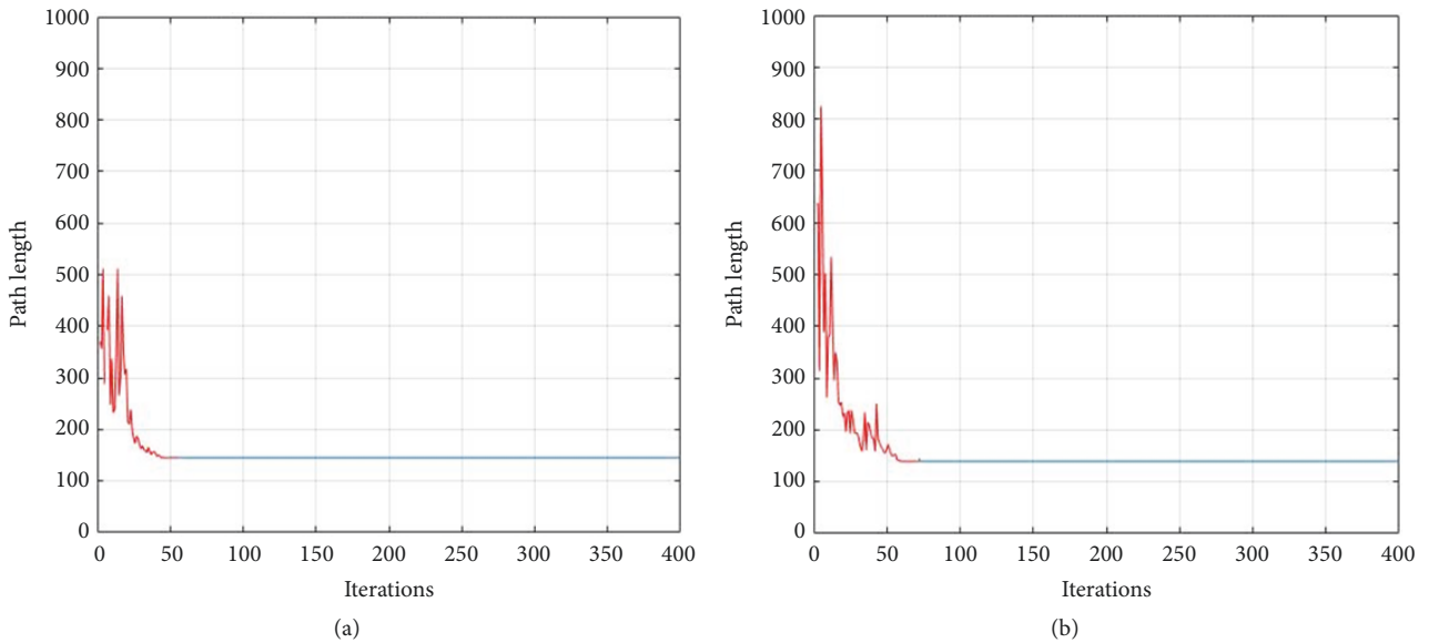
FIGURE 7: The optimal path length with the increase of iterations in another environment. There are both static and mobile threats in (a) and only mobile threats in (b).
