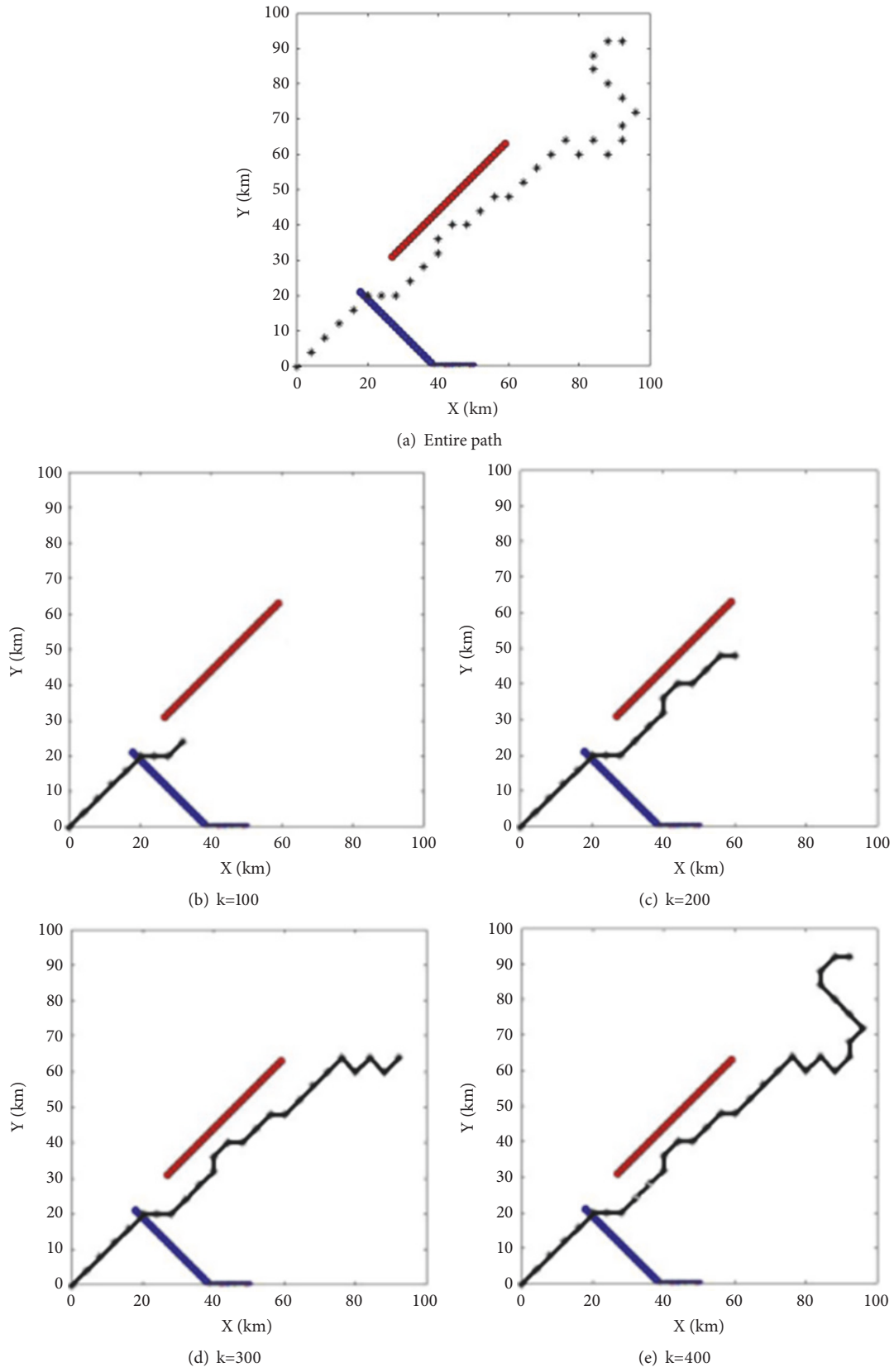
FIGURE 11: UAV path planning in one environment based on ACO algorithm. And there are only mobile threats where (a) is an entire path and (b) to (e) are paths with iterations = 100, 200, 300, 400.
