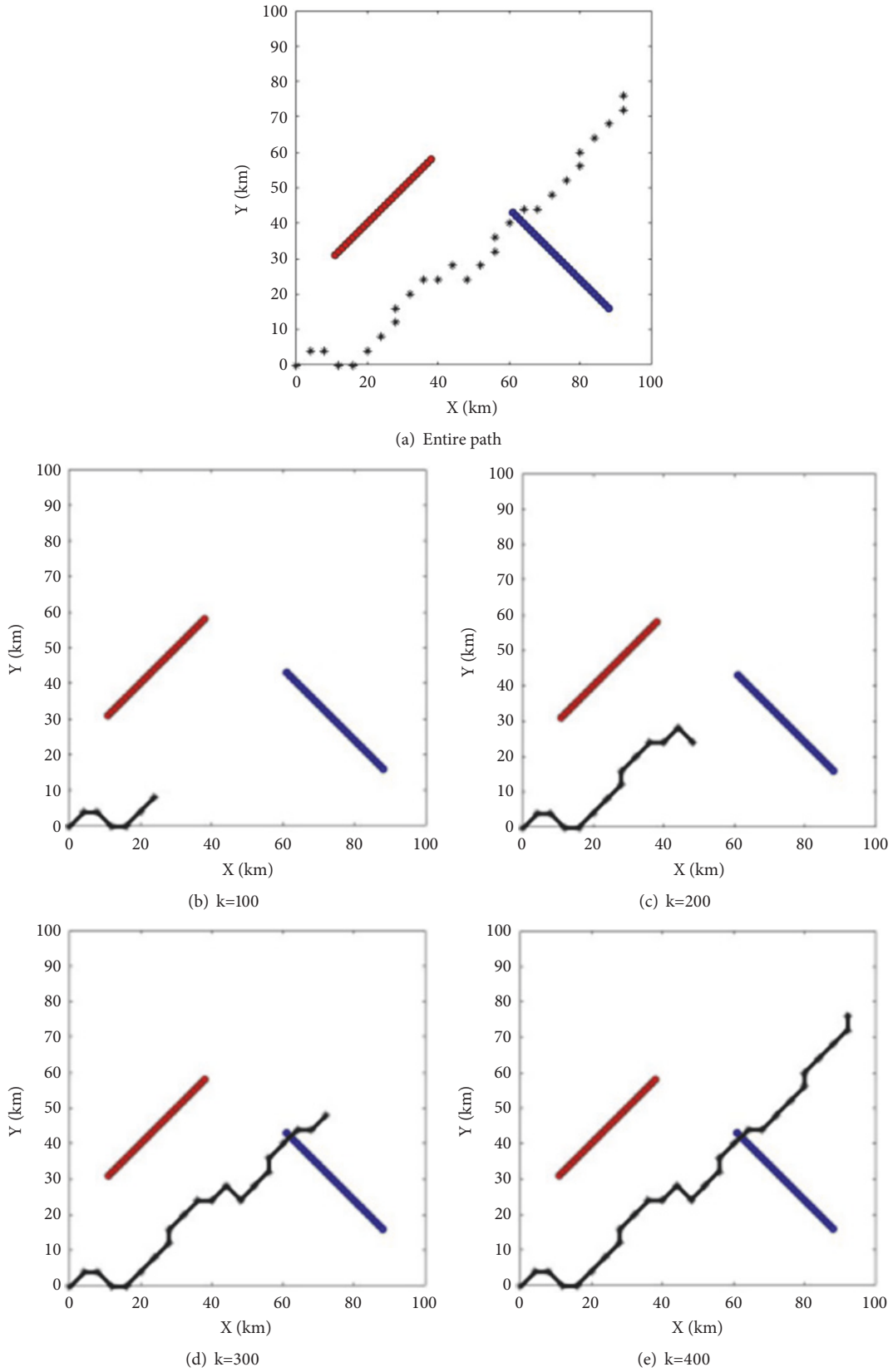
FIGURE 14: UAV path planning in another environment based on our proposed algorithm. And there are only mobile threats where (a) is an entire path and (b) to (e) are paths with iterations = 100, 200, 300, 400.
