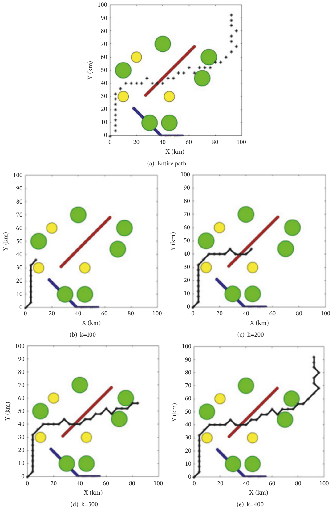
FIGURE 9: UAV path planning in one environment based on ACO algorithm. And there are both static and mobile threats where (a) is an entire path and (b) to (e) are paths with iterations = 100, 200, 300, 400.
