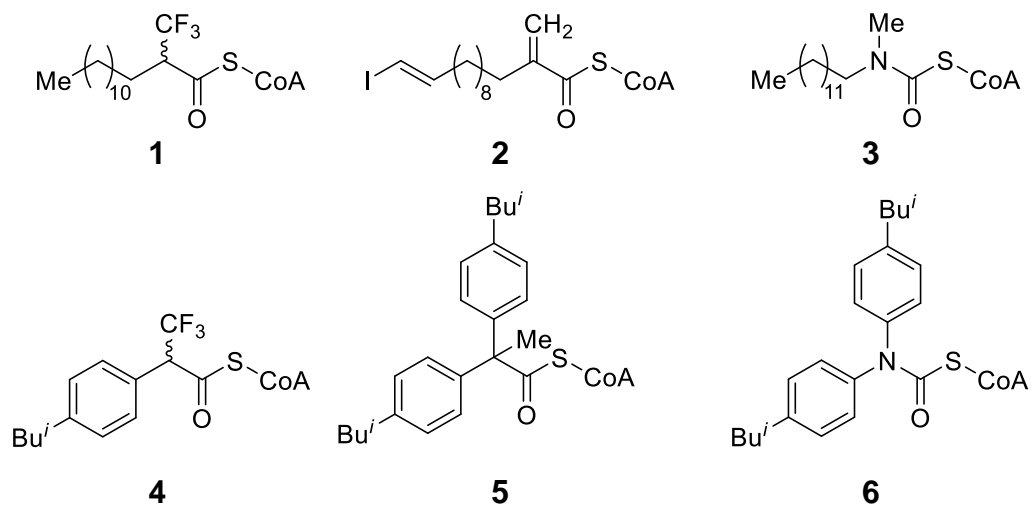
Figure 1: Examples of previously reported rationally designed AMACR inhibitors 1 - 4 [29-32] and inhibitors 5 and 6 of MCR [33, 34], the M. tuberculosis homologue of AMACR.
