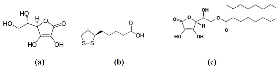
Figure 1. Chemical structures of ascorbic acid (a), lipoic acid (b) and ascorbyl palmitate (c).
