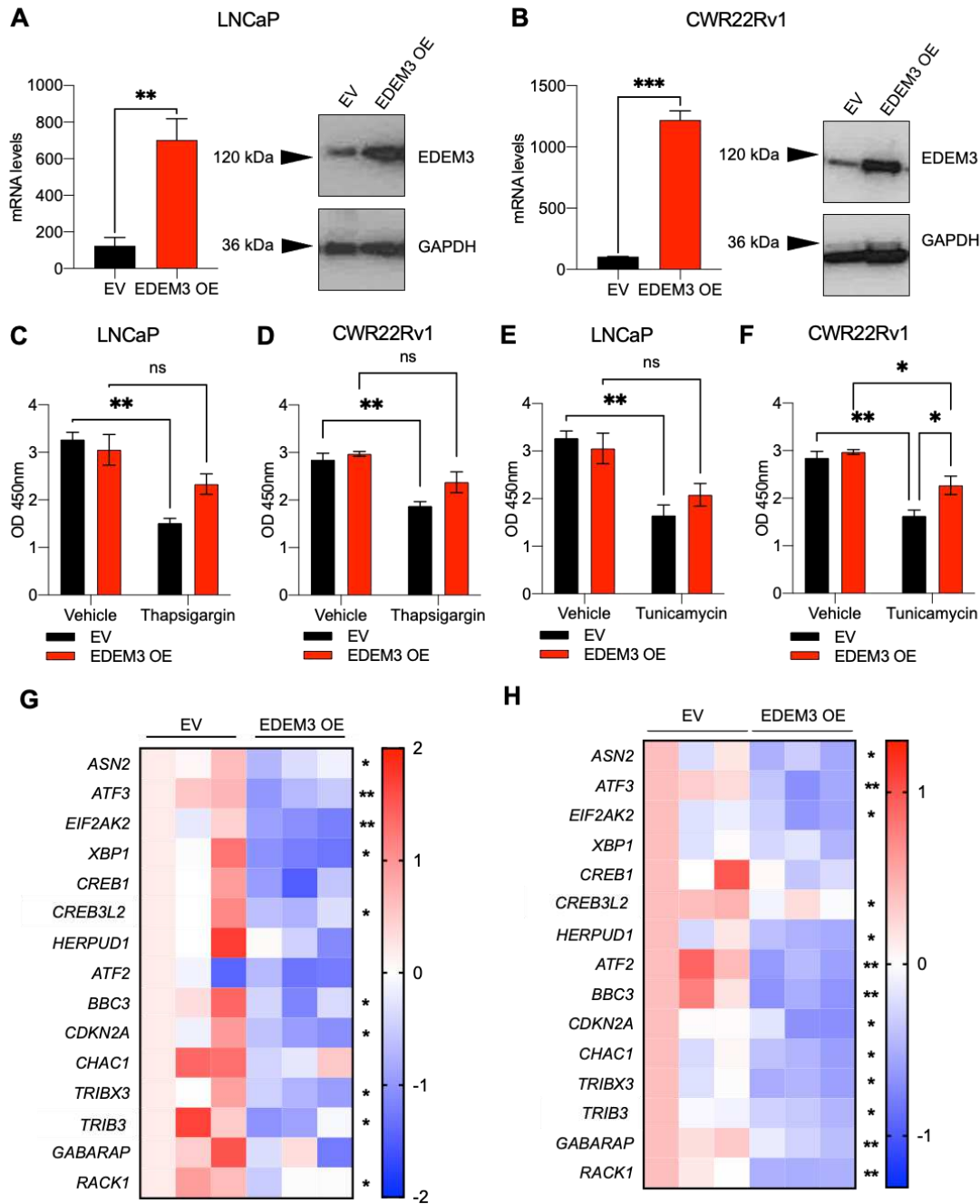
Figure 4. EDEM3 overexpression in prostate cells protects from ER stressors (A-B) mRNA and protein levels of EDEM3 in LNCaP and CWR22Rv1 cells following overexpression of EDEM3 compared with an empty vector control. Data are presented as mean \pm s.e.m. Western blot analysis shown with GAPDH used as a loading control. (C-F) Cellular viability of LNCaP and CWR22Rv1 cells, with overexpression of EDEM3, treated with either vehicle (DMSO), 2.5 \mu M tunicamycin or 100 nM thapsigargin for 24 hours. Viability measured by WST-1 assay and shown as absorbance at O.D 450 nm. N=3. Data are mean \pm s.e.m. P values were calculated using two tailed unpaired t-tests. * P < 0.05, ** P < 0.01 and *** P < 0.001. (G-H) Heatmap showing mRNA levels of ASN2 , ATF3 , EIF2AK3 , XBP1 , CREB1 , DDIT3 , HERPUD1 , ATF2 , BBC3 , CDKN2A , CHAC1 , TRIBX3 , DDIT4 , GABARAP and RACK1 in LNCaP (G) and CWR22Rv1 (H) cells following overexpression of EDEM3 compared with empty vector control. N=3 and data are presented as z-scores. P values were calculated using two tailed unpaired t-tests. * P < 0.05, ** P < 0.01 and *** P < 0.001.
