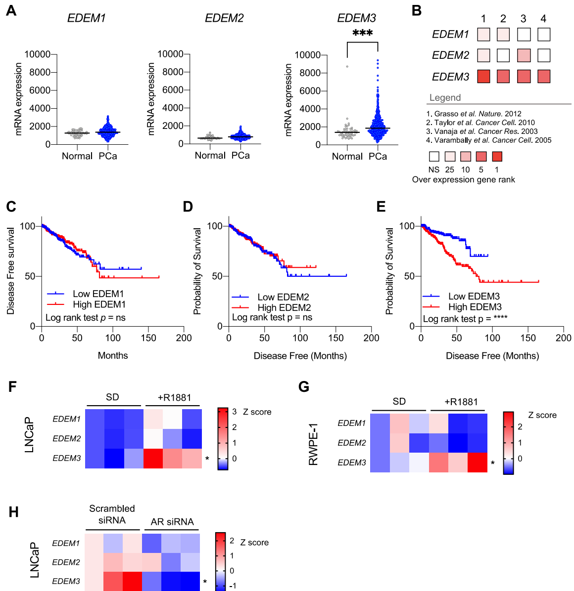
Figure 1. EDEM3 up-regulation is associated with a reduced disease-free survival in prostate cancer (PCa). (A) Analysis of EDEM gene expression in The Cancer Genome Atlas (TCGA) prostate adenocarcinoma cohort (N=497) compared with normal prostate samples (52). (B) Meta-analysis of EDEM1/2/3 gene expression in prostate cancer. Four independent prostate cancer gene expression data sets (N=366) were analysed for EDEM1/2/3 gene expression in prostate cancer patients compared with patients with normal. Data shown is of overexpression gene rank in each dataset. Legend includes details of the independent cohorts. NS = not significant, 25 = top 25%, 10 = top 10%, 5 = top 5% and 1 = top 1%. Data accessed using OncoPrint 27-30 . (C-E) Kaplan-Meier plot showing disease free survival for prostate cancer patients stratified based on low (bottom 50%) or high (top 50%) EDEM3 expression. Analysis includes 471 prostate cancer patients from TCGA PRAD cohort, accessed via CBioPortal. P value was calculated by log rank test. (F-G) Heatmaps showing mRNA levels of EDEM1/2/3 in both LNCaP and RWPE-1 cultured in either steroid depleted (SD) conditions or stimulated with 10 nM R1881 for 24 hours. N=3 and data are presented as z-scores. (H) Heatmap showing mRNA levels of EDEM1/2/3 in LNCaP cells following androgen receptor siRNA knockdown, compared with scrambled siRNA control. N=3 and data are shown as z-scores. P values were calculated using a two tailed unpaired t-test. *P < 0.05, **P < 0.01 and ***P < 0.001.
