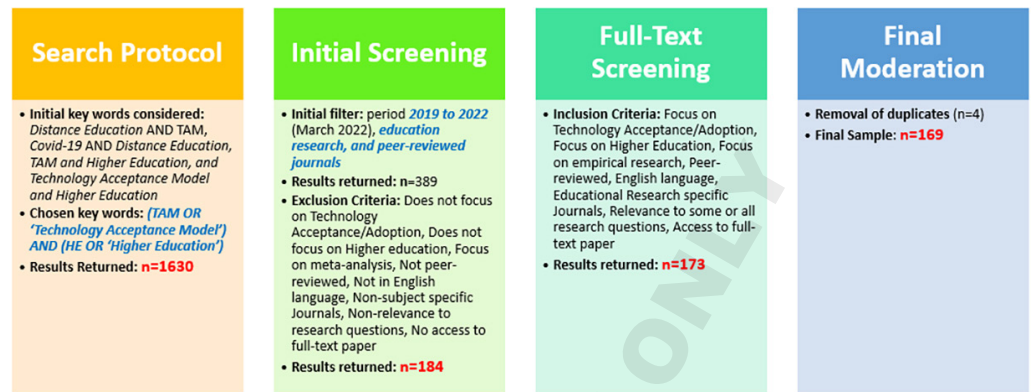
Fig. 1. Screening process
