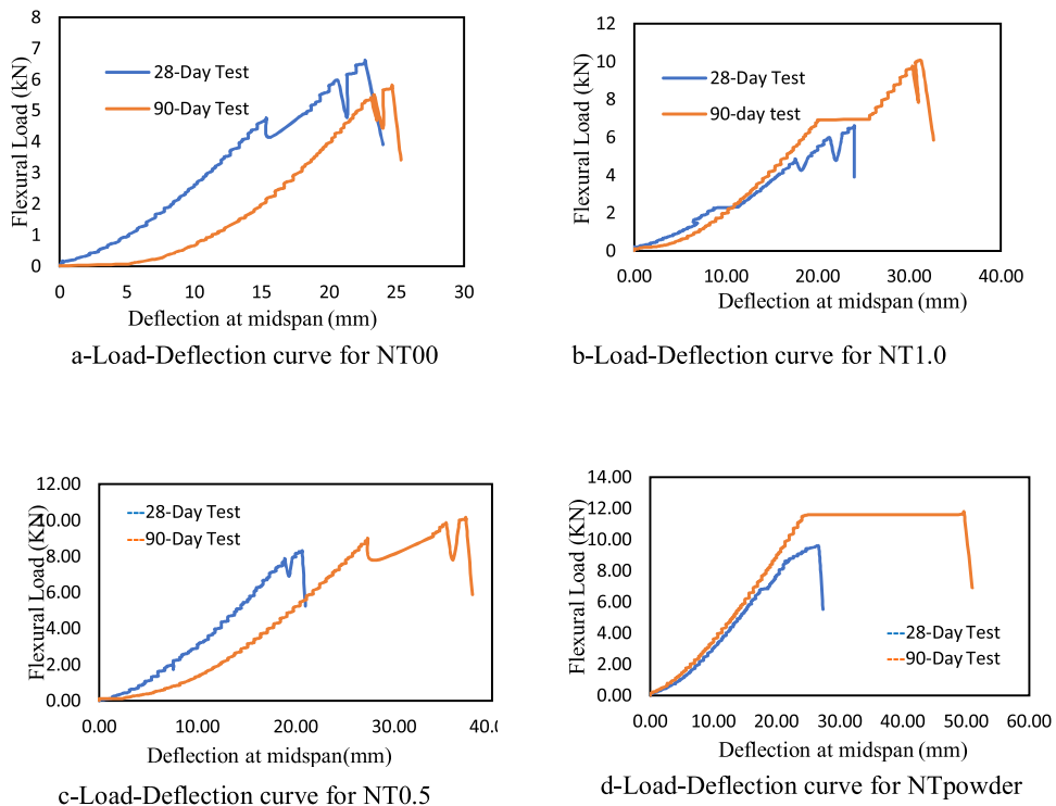
Fig. 7. a - Load-Deflection curve for NT00 Fig. 7b-Load-Deflection curve for NT1.0. Fig. 7c -Load-Deflection curve for NT0.5. Fig. 7d -Load-Deflection curve for NTpowder.
