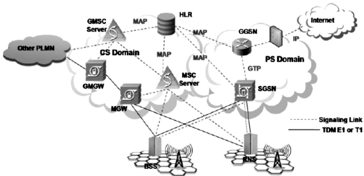
Figure 3. UMTS release 4 Core Network Architecture
