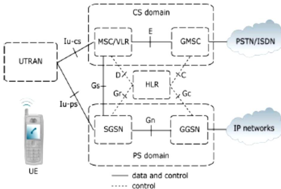
Figure 2. UMTS Release 99 Architecture
