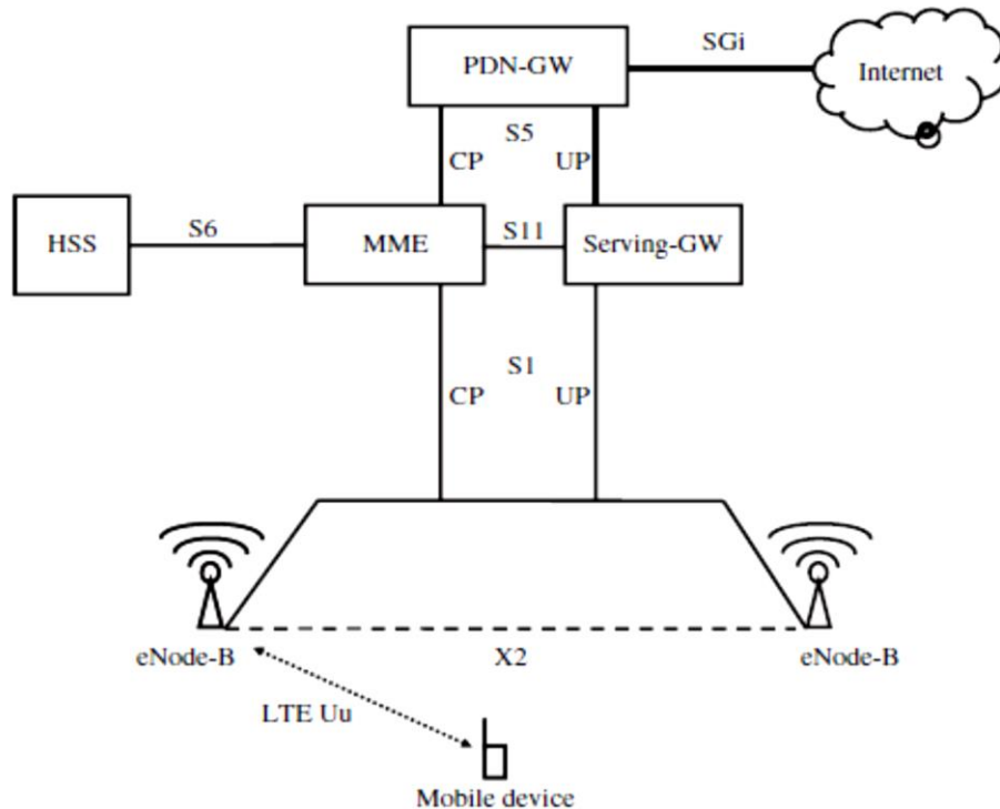
Figure 4. LTE Network Overview
