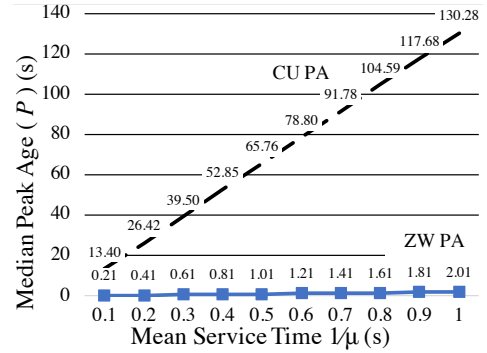
Fig. 6. ZW and CU, PA performance ( P ) versus service time for S1. The PA value for both policies increase with the service time, however, its value for CU is notably higher.
