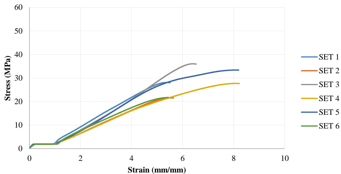
Figure 8. Laminates only
